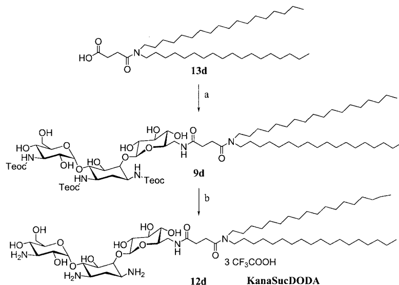
Scheme 4. Synthesis of KanaSudDODA. a) HOAt/EDC, 4 , DMF/CH 2 Cl 2 ; b) CF 3 CO 2 H
